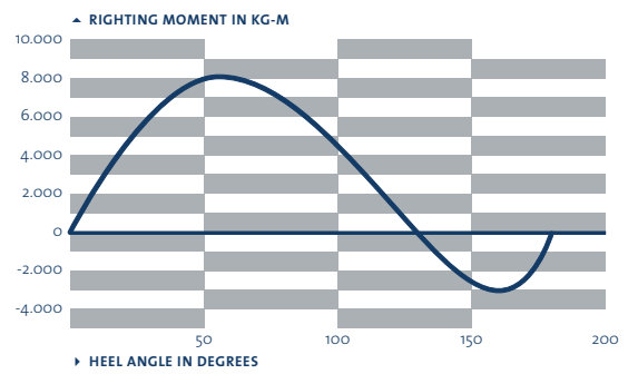
STABILITY CURVE
