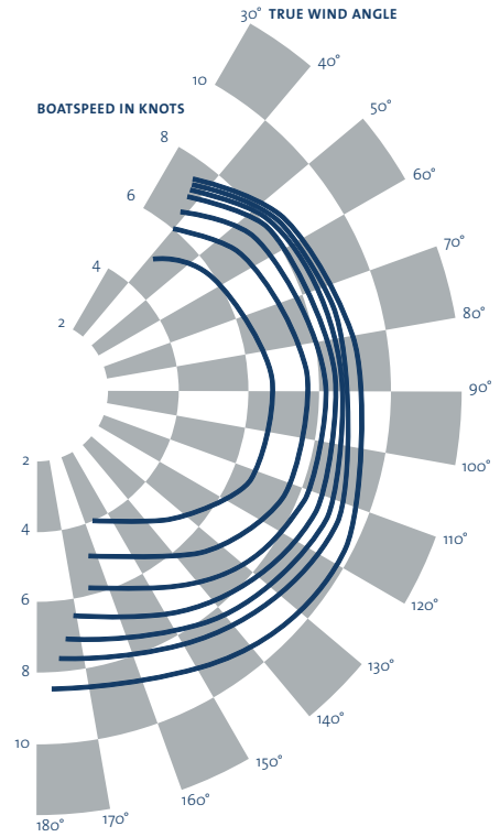
POLAR PERFORMANCE DIAGRAM
